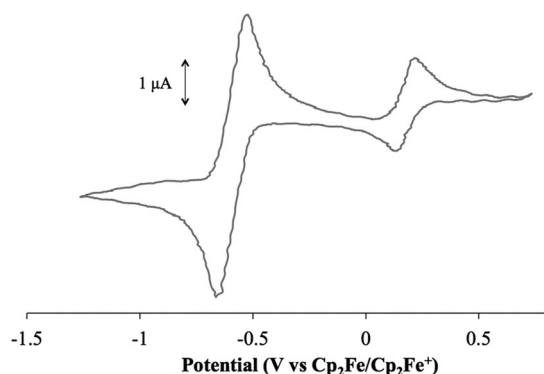
Figure 2. Cyclic voltammogram of 12\text{-}[\text{Cp}^*_2\text{Fe}]^+ in 0.1 M [\text{nBu}_4\text{N}]^+[\text{PF}_6]^- in \text{CH}_2\text{Cl}_2 recorded with a glassy carbon electrode. Scan rate 50 \text{ mV s}^{-1} . Potentials referenced to \text{Cp}_2\text{Fe}/\text{Cp}_2\text{Fe}^+ .
